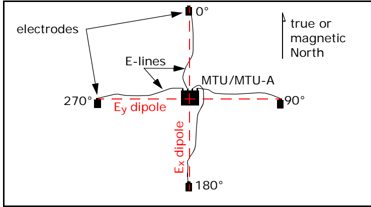
Fig. 1-2: Standard site layout.
