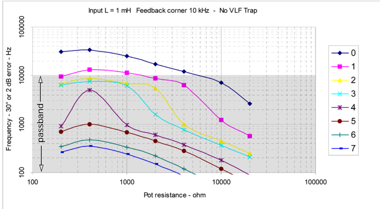
Fig. 4-7: Response curves for AMT (10kHz feedback corner frequency) with VLF trapping Off.
