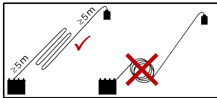
Fig. 1-5: Lay excess cable in S-shapes, not coils.
