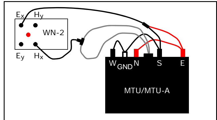
Fig. C-4: Setup for parallel white noise test. (Battery and GPS antenna omitted for clarity.)
