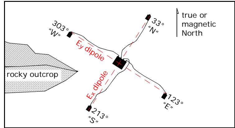
Fig. 1-4: Site rotated to avoid an obstruction.
