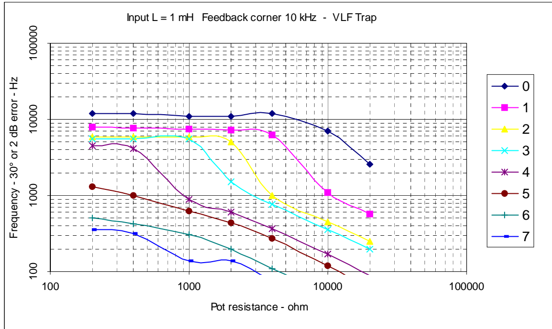
Fig. 4-6: Response curves for AMT (10kHz feedback corner frequency) with VLF trapping On.
