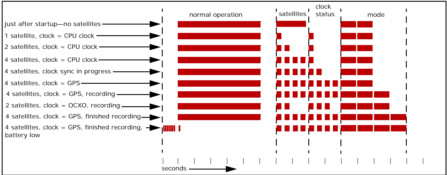
Fig. 2-35: Example of how the pattern might change during a normal sounding. At first there are no satellites acquired, then 1 satellite, then 2, then 4 or more. As satellites are acquired, the clock synchronizes first with the CPU, then with GPS/UTC. At the programmed start time, the mode changes from standby to record mode. Satellites may be lost temporarily, leaving the clock synchronized to the OCXO while recording continues. Recording stops at the programmed time and the instrument idles, possibly draining the battery below 11V.
