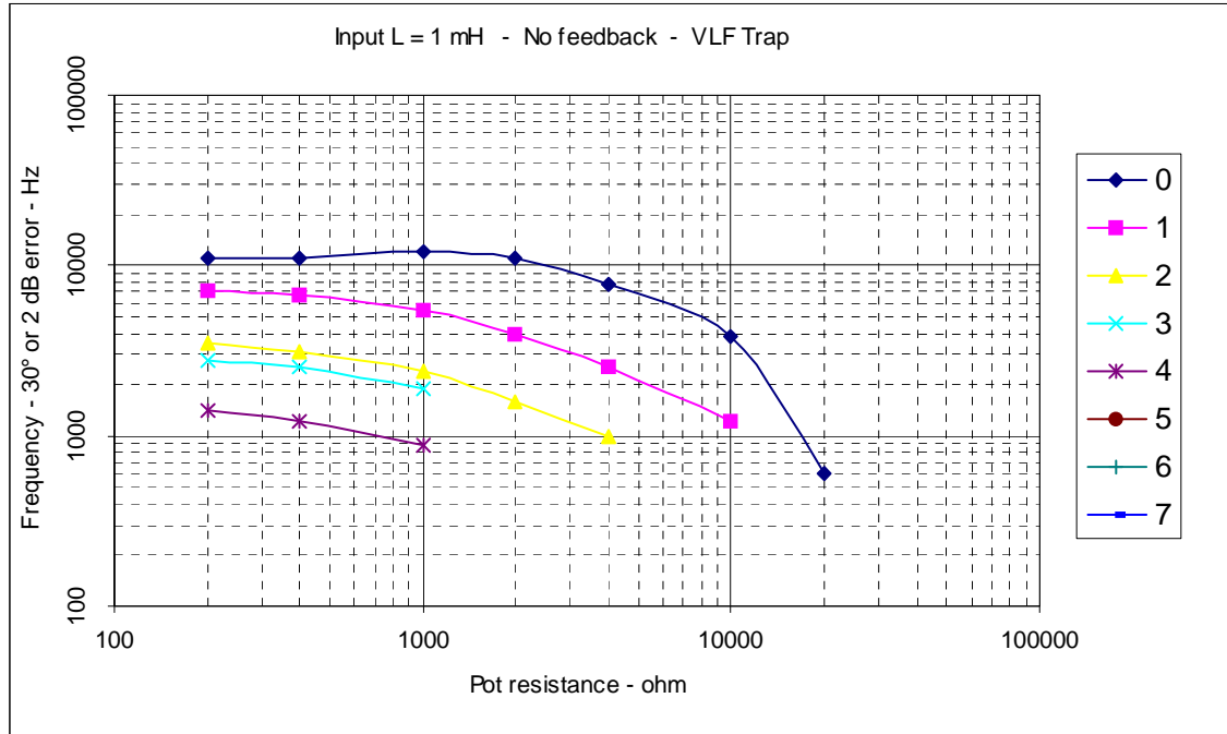
Fig. 4-5: Response curves for broadband (no feedback corner frequency) with VLF trapping On.
