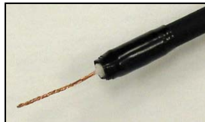
Fig. 2-7: An E-line cable stripped and wrapped with electrician's tape.
