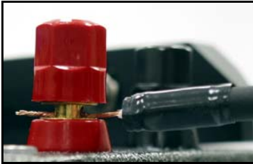
Fig. 2-8: E-line cable threaded through the MTU terminal shaft. Wrap the free end around the shaft before tightening the terminal.
