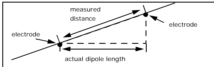
Fig. 1-6: Side view of a hill shows the effect of slope on dipole length.
