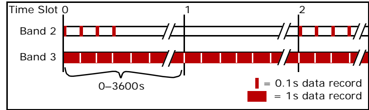
Fig. 4-3: MTU-A sampling scheme ("Dense" AMT data).
