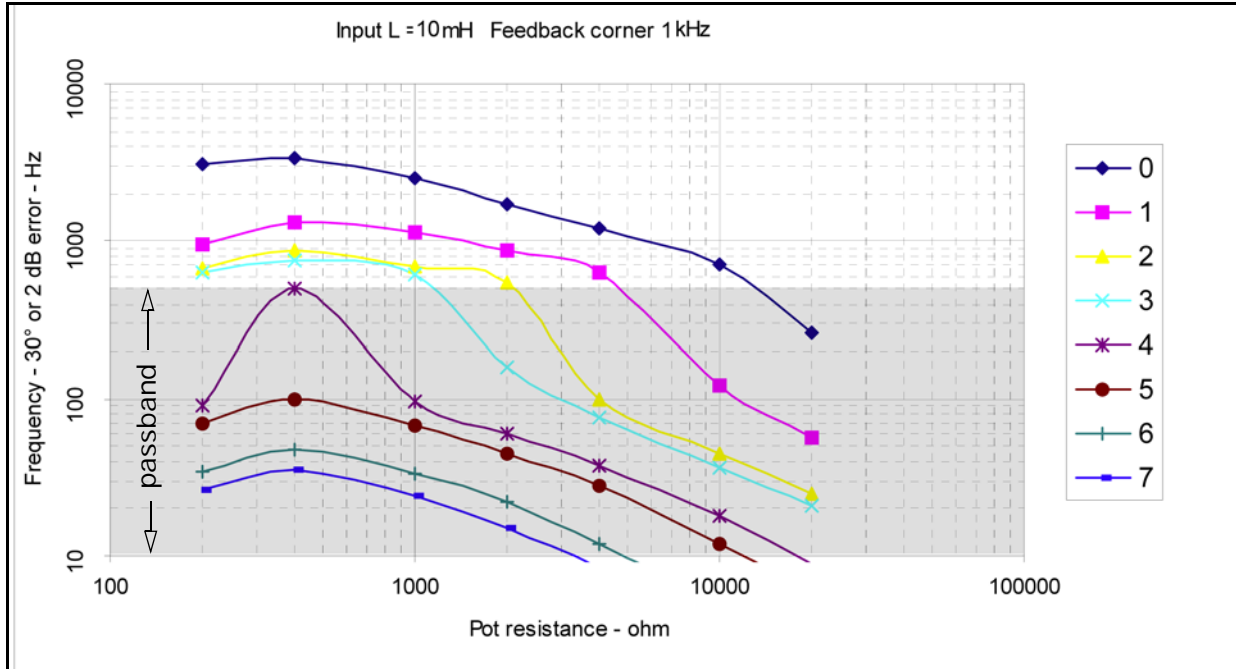
Fig. 4-8: Response curves for MT (1kHz feedback corner frequency) with VLF trapping Off.
