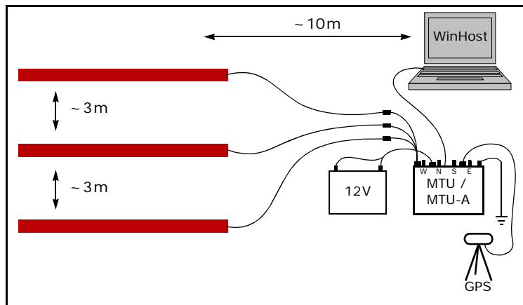
Fig. 2-36: Coil calibration layout.
