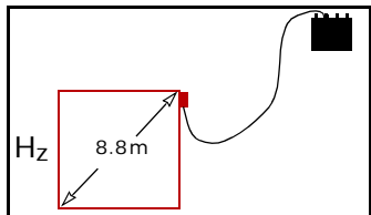
Fig. 2-47: Air-loop cable must exit the pre-amplifier toward the right when viewed from within the air-loop.
