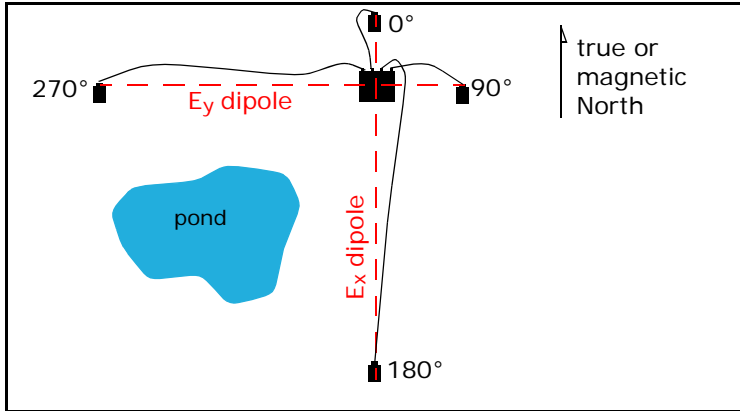
Fig. 1-3: E-line lengths adjusted to avoid an obstruction.
