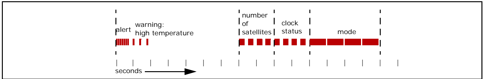
Fig. 2-33: Example of idling after acquisition with internal temperature exceeding 60°C.
