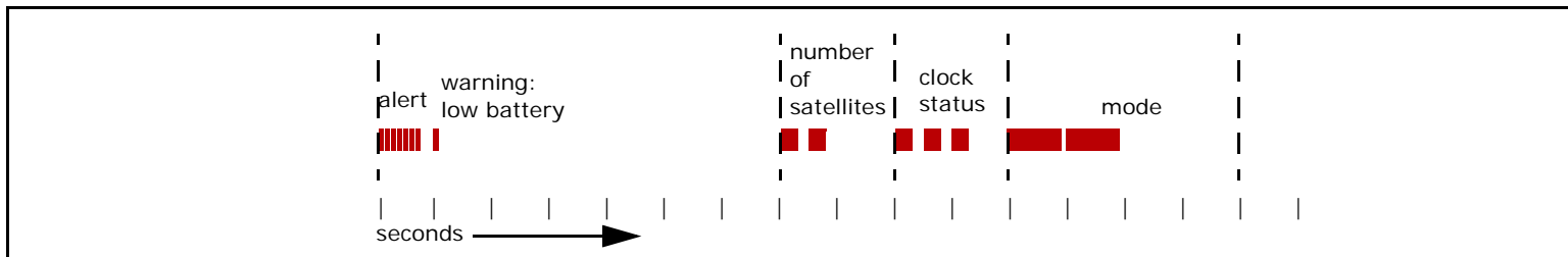
Fig. 2-34: Example of operation in standby mode when synchronized to OCXO, with a low battery warning.
