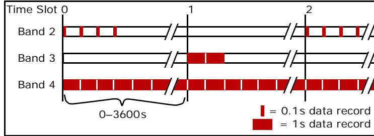
Fig. 4-1: MTU-A sampling scheme (AMT data and AMT-compatible MT data).
