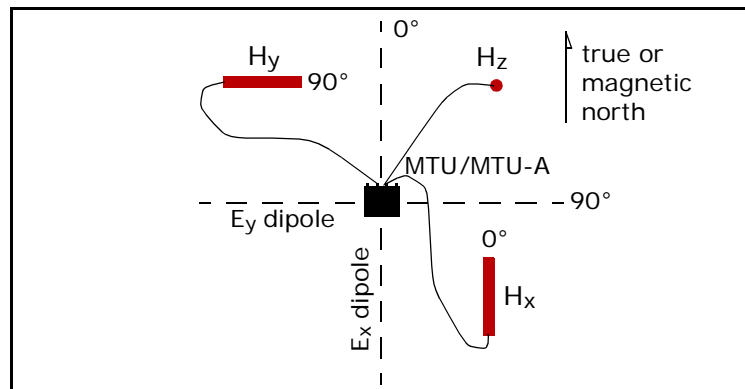
Fig. 1-7: Example layout with three coils correctly oriented (not to scale).
