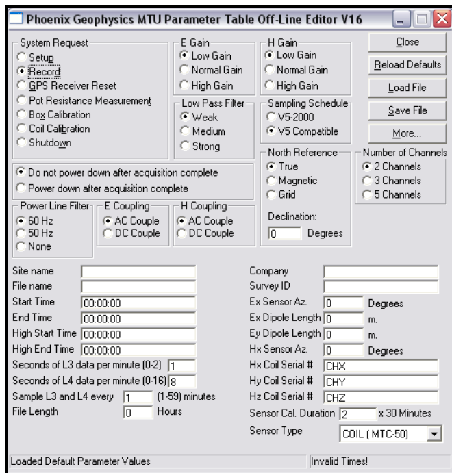
Fig. 3-1: WinTabEd main window.
