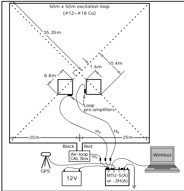
Fig. 2-39: Air-loop sensor calibration.
