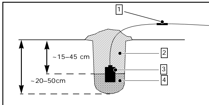
Fig. 2-42: Side view of electrode installation. (1) Electrode cable spliced to E-line and wrapped with electrical tape; (2) loose dirt to cover electrode; (3) electrode; (4) salty mud mixture.
