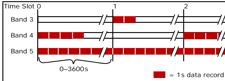
Fig. 4-2: MTU-A sampling scheme (MT data).
