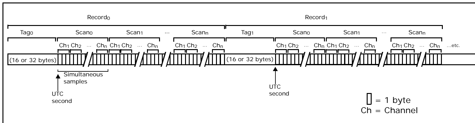
Figure G-1: A graphical representation of the time series file format. The scans within one record span either one second (Bands 3, 4, and 5) or 0.1 second (Band 2). Records always begin on a UTC second, but not necessarily on consecutive UTC seconds.
