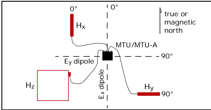
Fig. 1-8: Example layout with two coils and an air-loop correctly oriented (not to scale).
